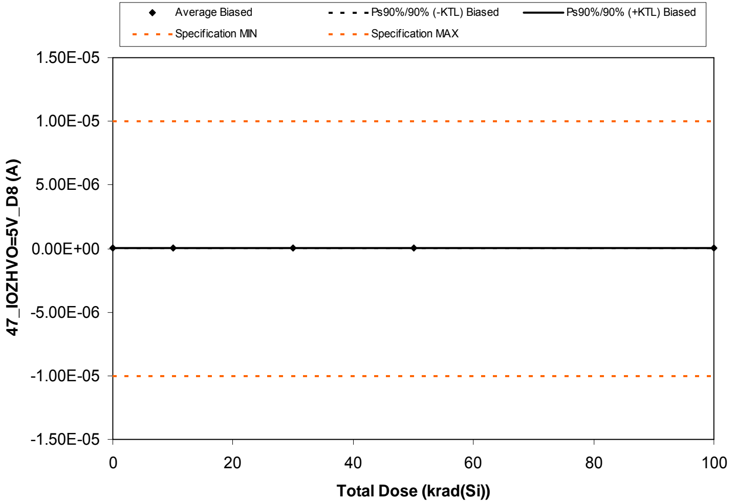
Figure 5.45. Plot of 47\_IOZHVO=5V\_D8 (A) versus total dose. The solid diamonds are the average of the measured data points for the samples irradiated under electrical bias and the black lines (solid and/or dashed) are the average of the data points after application of the KTL statistics on the samples irradiated under electrical bias. The red dotted line(s) are the pre- and/or post-irradiation minimum and/or maximum specification value as defined in the datasheet and/or test plan.
