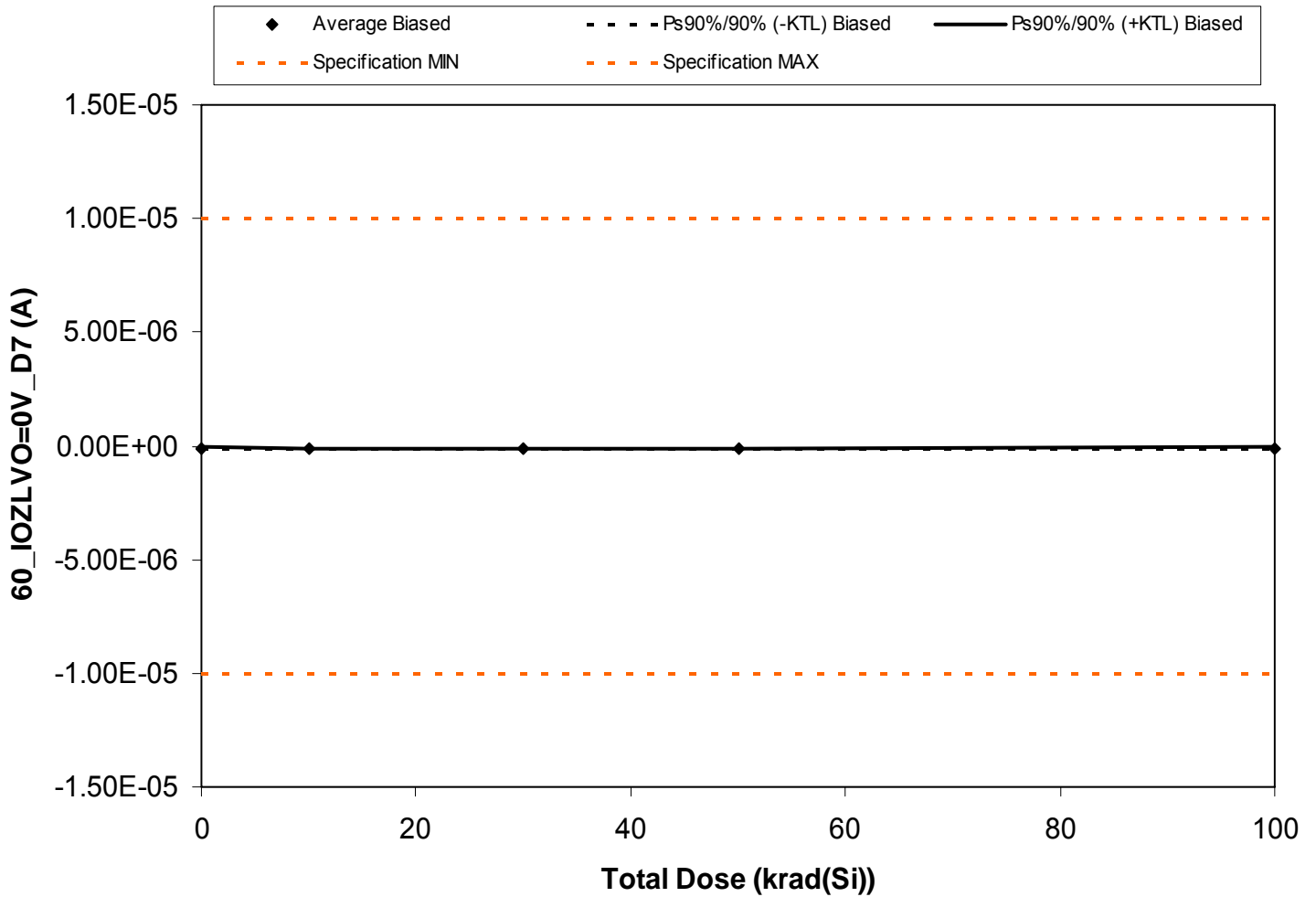
Figure 5.58. Plot of 60_IOZLVO=0V_D7 (A) versus total dose. The solid diamonds are the average of the measured data points for the samples irradiated under electrical bias and the black lines (solid and/or dashed) are the average of the data points after application of the KTL statistics on the samples irradiated under electrical bias. The red dotted line(s) are the pre- and/or post-irradiation minimum and/or maximum specification value as defined in the datasheet and/or test plan.
