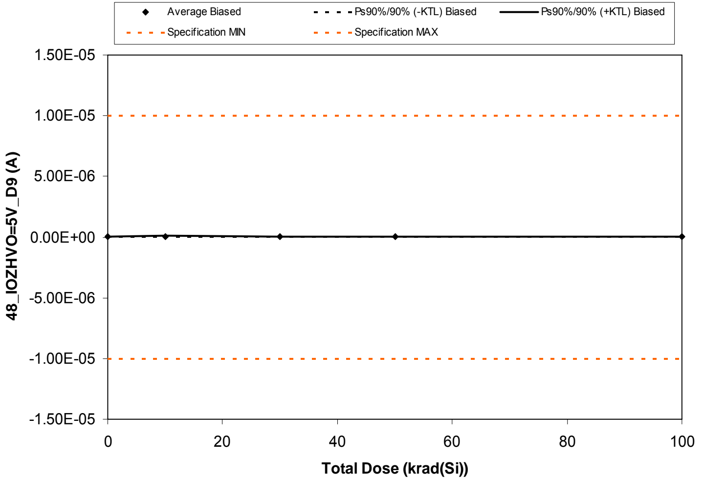
Figure 5.46. Plot of 48\_IOZHVO=5V\_D9 (A) versus total dose. The solid diamonds are the average of the measured data points for the samples irradiated under electrical bias and the black lines (solid and/or dashed) are the average of the data points after application of the KTL statistics on the samples irradiated under electrical bias. The red dotted line(s) are the pre- and/or post-irradiation minimum and/or maximum specification value as defined in the datasheet and/or test plan.
