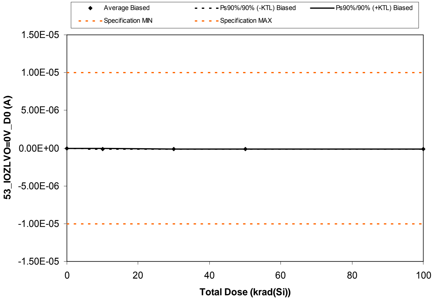
Figure 5.51. Plot of 53\_IOZLVO=0V\_D0 (A) versus total dose. The solid diamonds are the average of the measured data points for the samples irradiated under electrical bias and the black lines (solid and/or dashed) are the average of the data points after application of the KTL statistics on the samples irradiated under electrical bias. The red dotted line(s) are the pre- and/or post-irradiation minimum and/or maximum specification value as defined in the datasheet and/or test plan.
