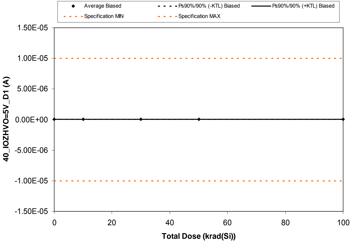
Figure 5.38. Plot of 40_IOZHVO=5V_D1 (A) versus total dose. The solid diamonds are the average of the measured data points for the samples irradiated under electrical bias and the black lines (solid and/or dashed) are the average of the data points after application of the KTL statistics on the samples irradiated under electrical bias. The red dotted line(s) are the pre- and/or post-irradiation minimum and/or maximum specification value as defined in the datasheet and/or test plan.
