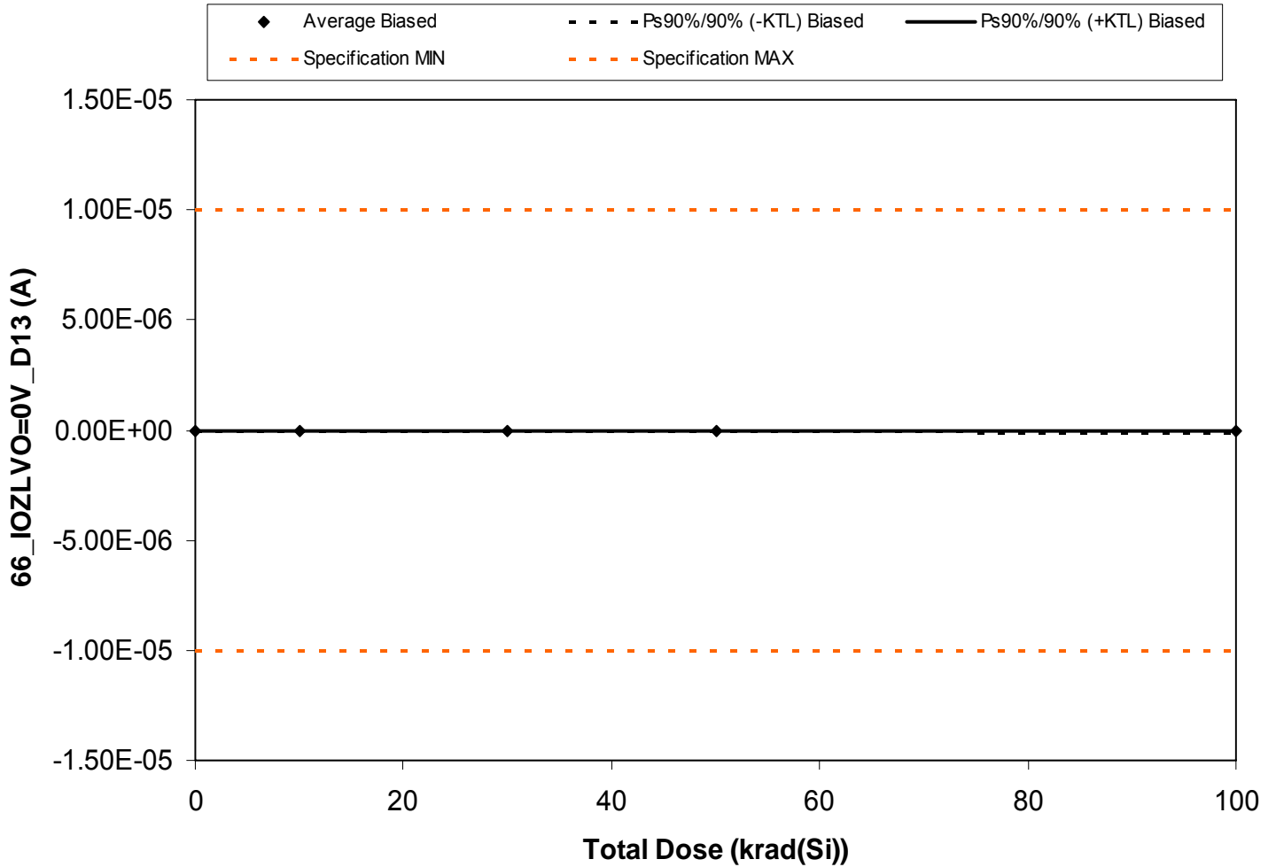
Figure 5.64. Plot of 66_IOZLVO=0V_D13 (A) versus total dose. The solid diamonds are the average of the measured data points for the samples irradiated under electrical bias and the black lines (solid and/or dashed) are the average of the data points after application of the KTL statistics on the samples irradiated under electrical bias. The red dotted line(s) are the pre- and/or post-irradiation minimum and/or maximum specification value as defined in the datasheet and/or test plan.
