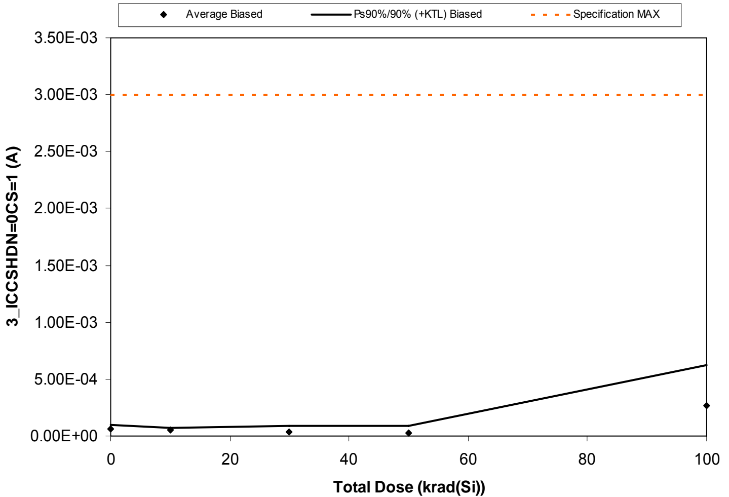
Figure 5.3. Plot of 3\_ICCSHDN=0CS=1 (A) versus total dose. The solid diamonds are the average of the measured data points for the samples irradiated under electrical bias and the black lines (solid and/or dashed) are the average of the data points after application of the KTL statistics on the samples irradiated under electrical bias. The red dotted line(s) are the pre- and/or post-irradiation minimum and/or maximum specification value as defined in the datasheet and/or test plan.
