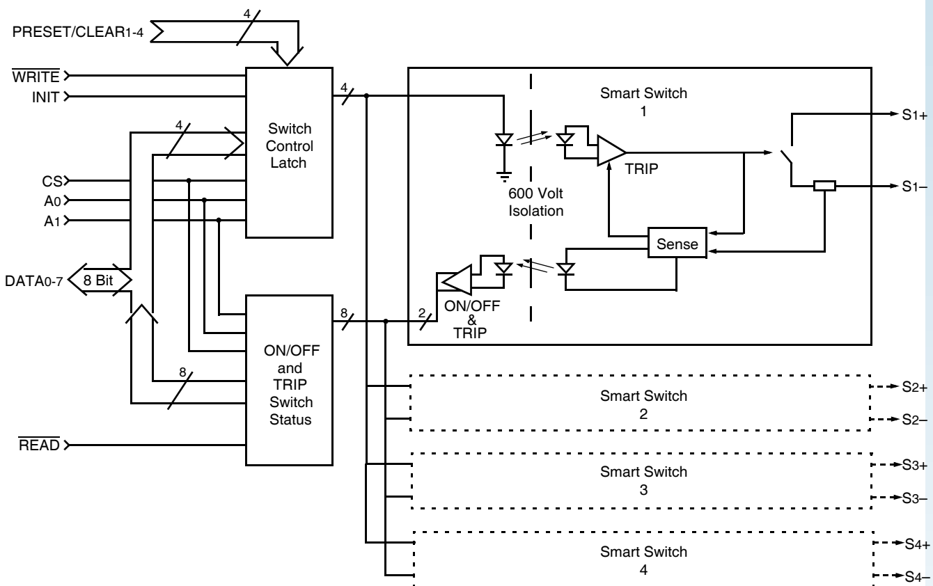
FIGURE 1 – Block Diagram
