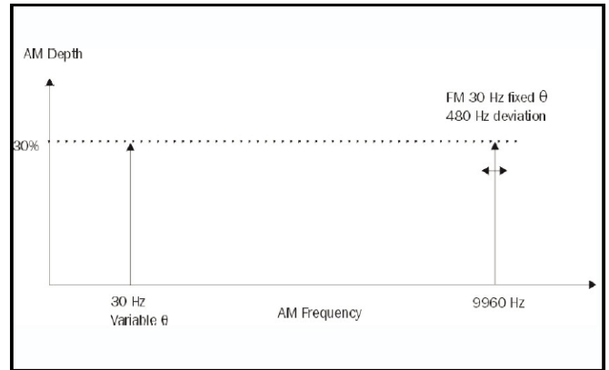
Figure 5 - Modulation Spectrum of a VOR Signal
