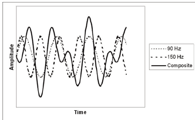
Figure 4 ILS waveform with the phase of the 150 Hz tone shifted by 180° compared to Figure 2.
