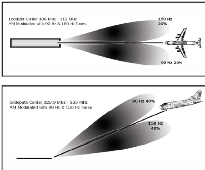
Figure 1 - Localizer and Glidescope systems of ILS installation
