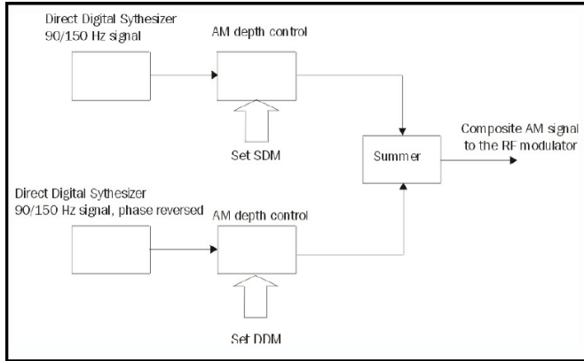
Figure 3 - Simplified schematic of the modulation drive system used in Option 6
