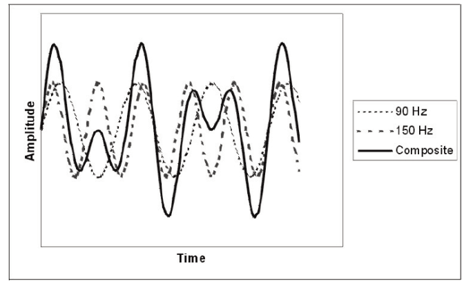
Figure 2 - ILS waveform with 0 DDM
