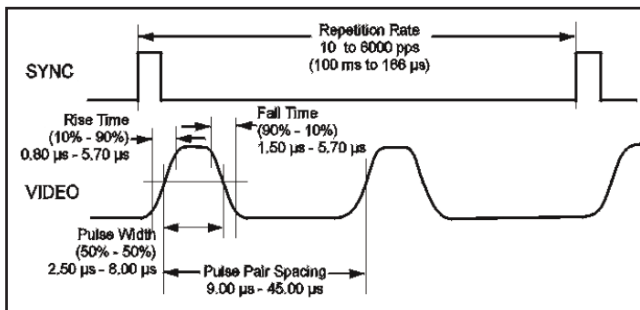
Figure 3 - Pulses definition in the 2030 signal generator
