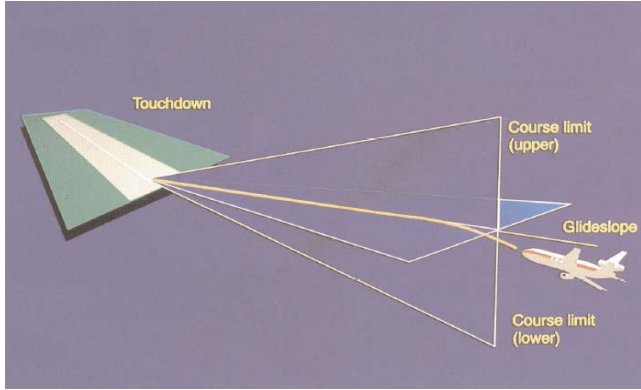
Figure 1 - Glideslope course width alarm limits
