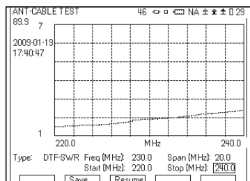
ANTENNA VSWR TEST
