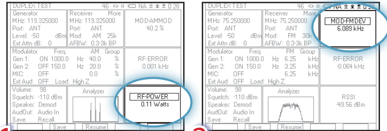
1 TRANSMITTER output power 2 TRANSMITTER deviation
