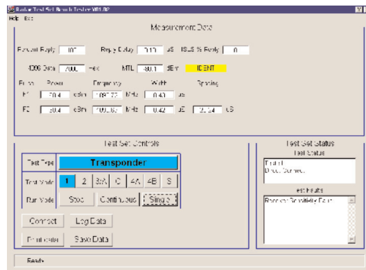
Transponder Test Screen (Shown in Mode S)
