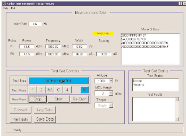
Interrogator Test Screen (Shown in Mode S)
