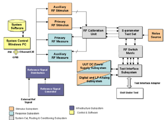
Figure 1. Generic Block Diagram of a SMART ^ E TM 5000 Environment Test Solution
